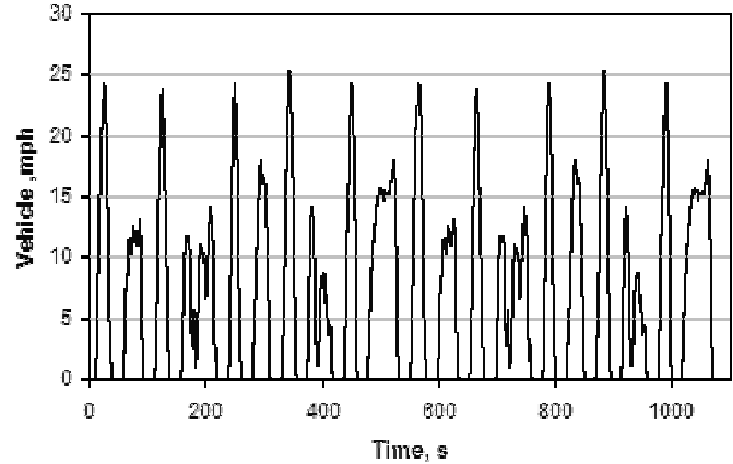
Figure 24. Manhattan Driving Cycle
