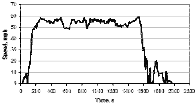
Figure 27. HHDDT Cruise Mode
