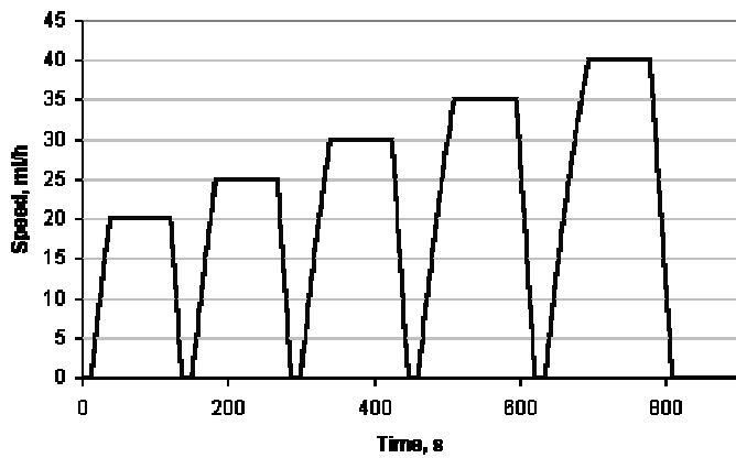
Figura 29. WVU 5-Peak
