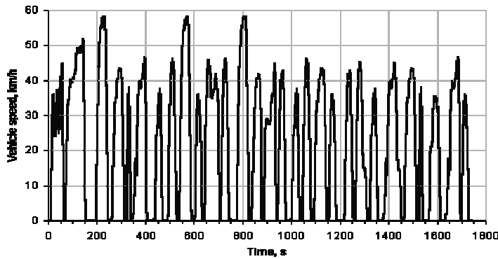
Figura 39. Braunschweig Cycle
