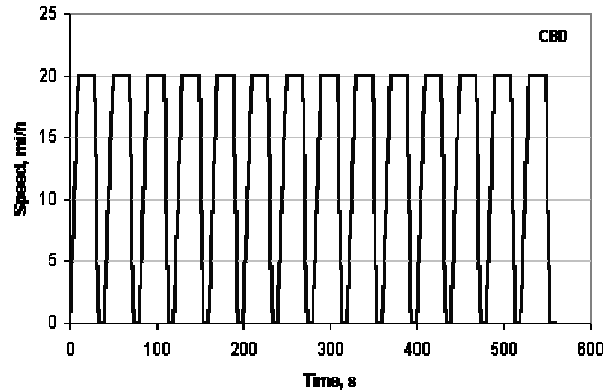
Figure 18. CBD Segment
