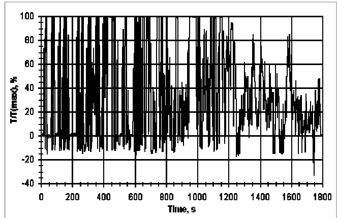
Figura 38. ETC Transient Cycle - Engine Torque
