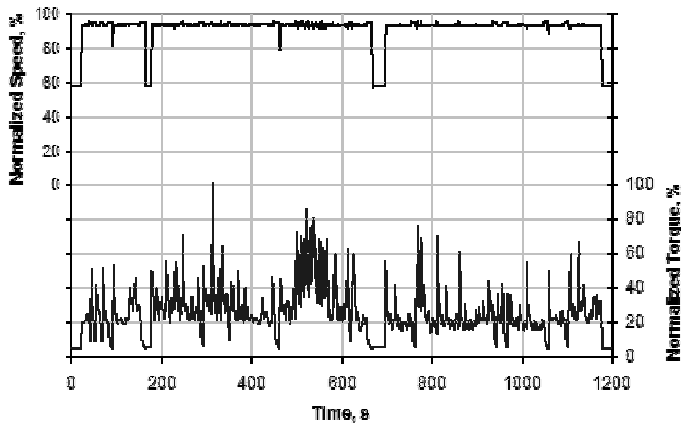
Figure 13. CSVL Cycle For Constant Speed Engines
