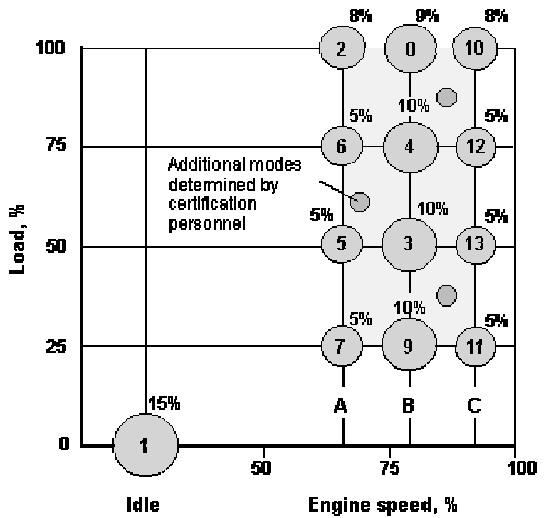
Figura 34. European Stationary Cycle (ESC)
