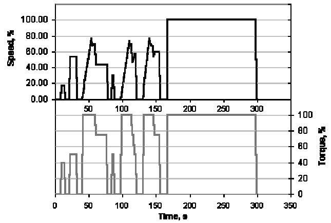
Figure 14. CTA Cycle
