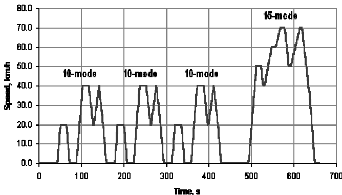
Figura 41. 10-15 Mode Cycle
