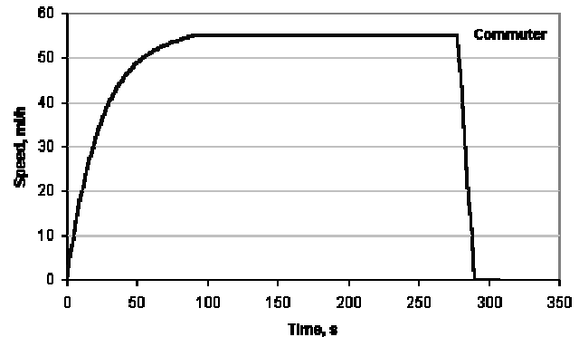
Figure 20. Commuter Segment
