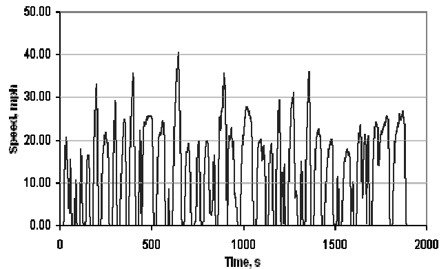
Figure 28. Orange County Bus Cycle
