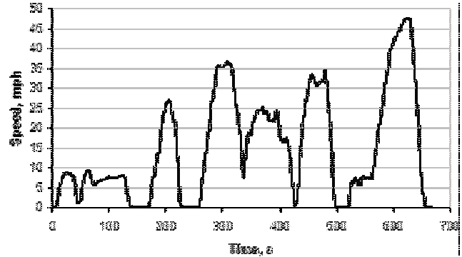
Figure 26. HHDDT Transient Mode
