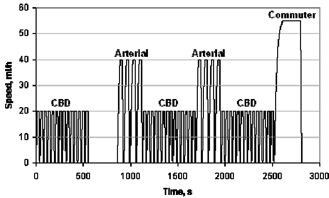
Figure 17. Composite BAC Cycle
