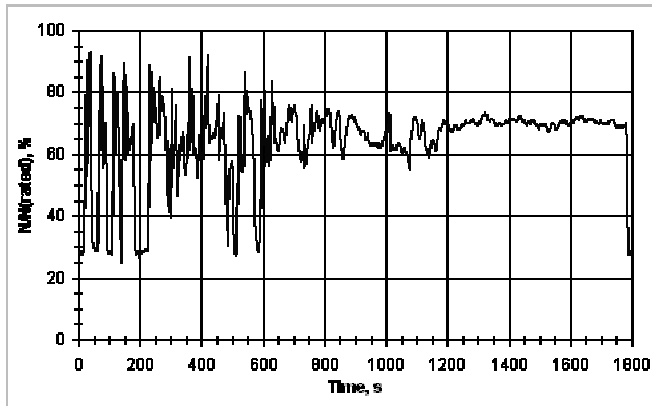
Figura 37. ETC Transient Cycle - Engine Speed
