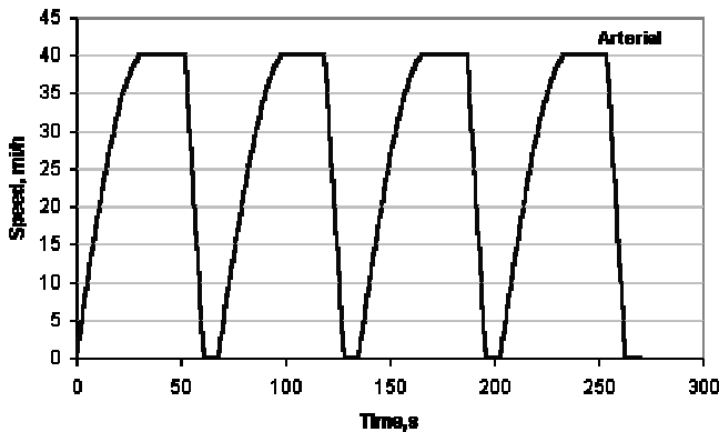
Figure 19. Arterial Segment
