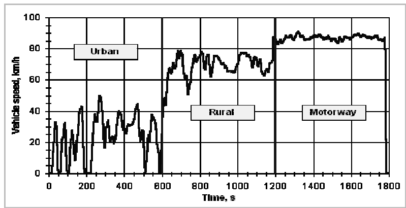
Figura 36. ETC Transient Cycle - Vehicle Speed
