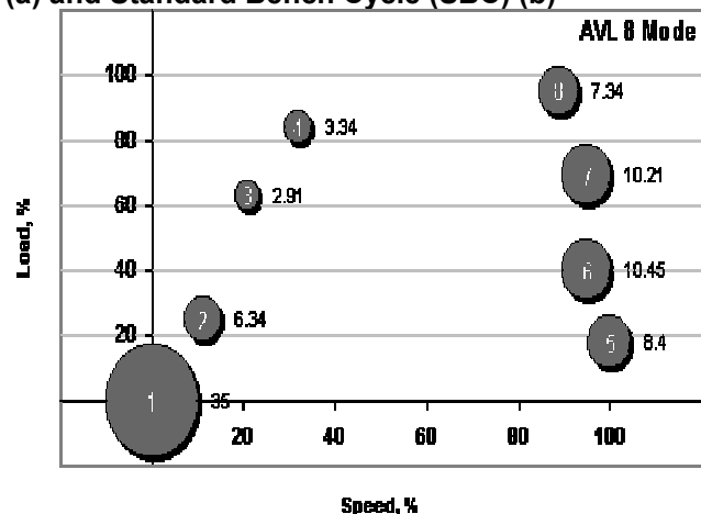
Figure 12. AVL 8-Mode Heavy-Duty Cycle
