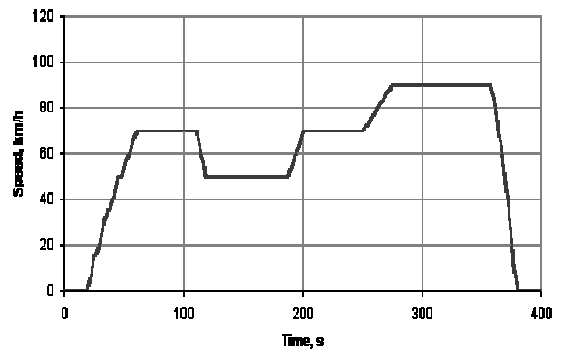
Figura 32. EUDC Cycle for Low Power Vehicles
